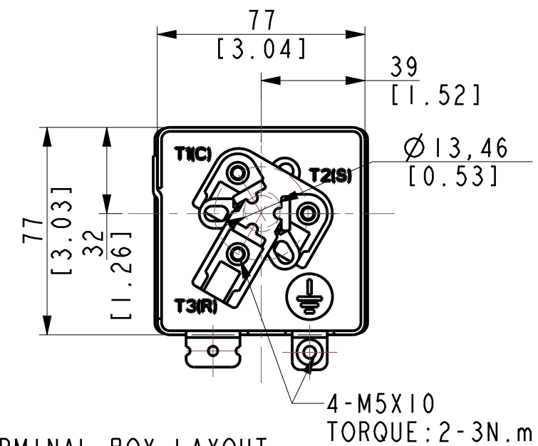
TERMINAL BOX LAYOUT SCALE 1:2
