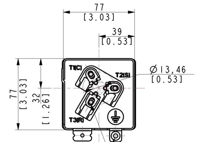
TERMINAL BOX LAYOUT SCALE 1:2 4-M5X10 TORQUE: 2-3N.m
