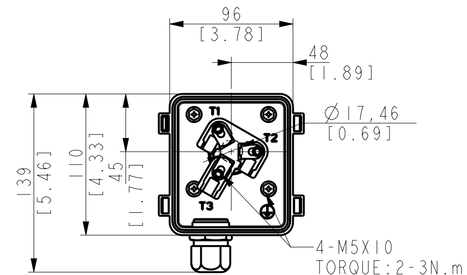
TERMINAL BOX LAYOUT SCALE 1:3
